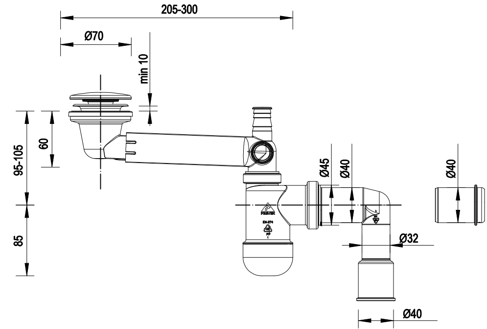
SPACE-SAVING SIPHON (Emporia-PR4-C4NNA-006)
