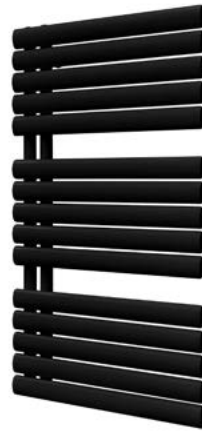
Bathroom radiator, 99x50 cm, power 551W, bottom power supply, installation kit included, black matt
