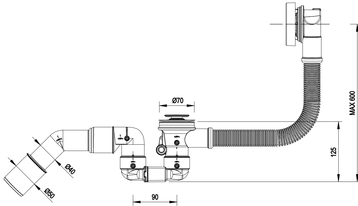
SIPHON (EMPORIA-BBL-R5R45-003)
