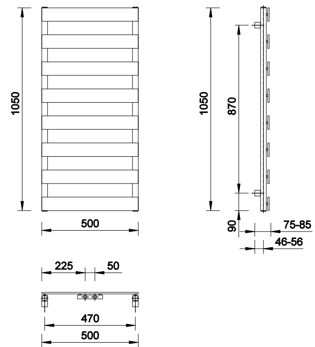
OTUS BOTTOM AND CENTRAL POWER SUPPLY 105x50 cm (EMPORIA-OTUS1050-500-CMZD | EMPORIA-OTUS1050-500-CMZDC)
