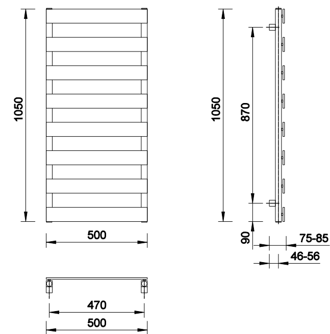
OTUS BOTTOM AND CENTRAL POWER SUPPLY 105x50 cm (EMPORIA-OTUS1050-500-CMZD | EMPORIA-OTUS1050-500-CMZDC)
